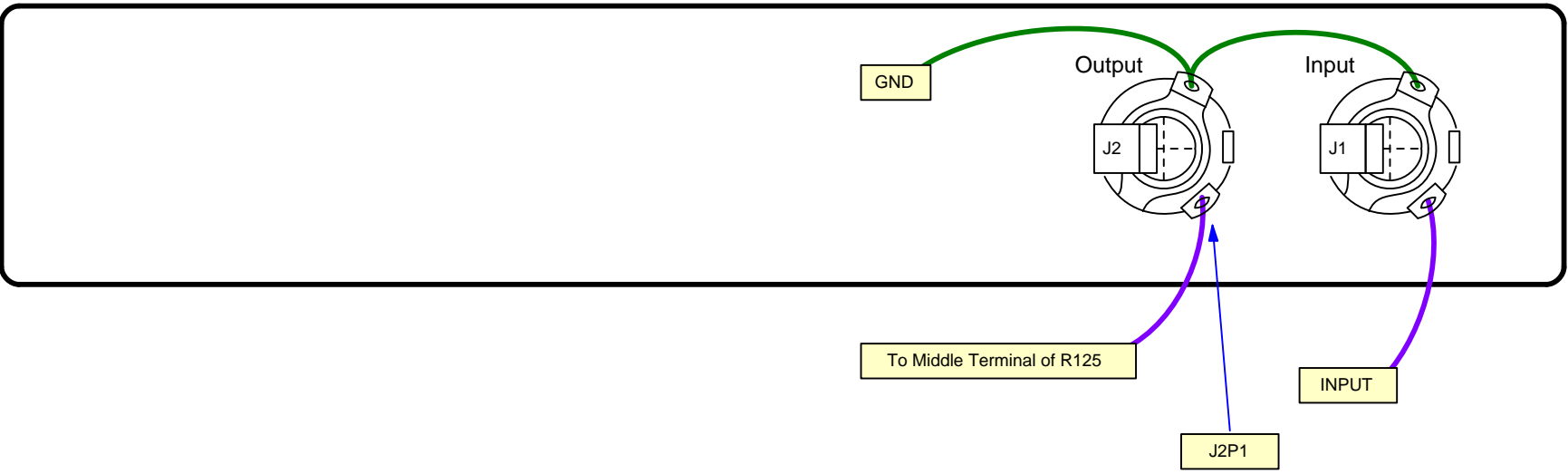
MFOS Sub-Commander Rear Panel Wiring View
