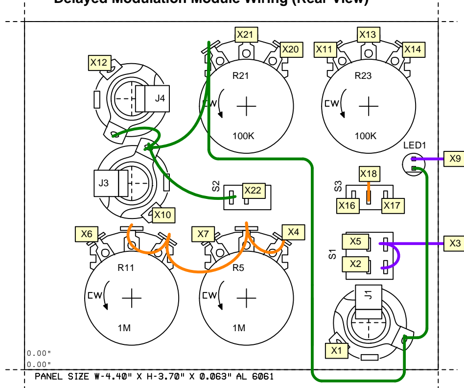
Delayed Modulation Module Wiring (Rear View)
