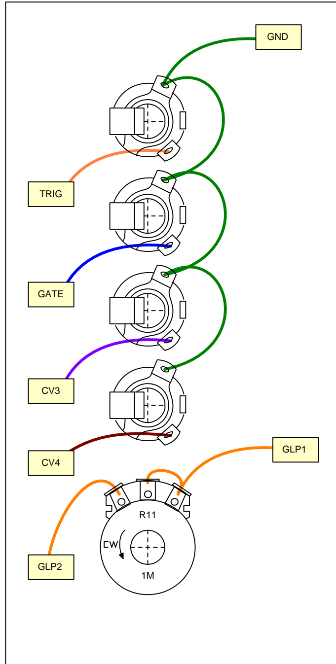
Mini-Controller Panel Wiring Rear View
