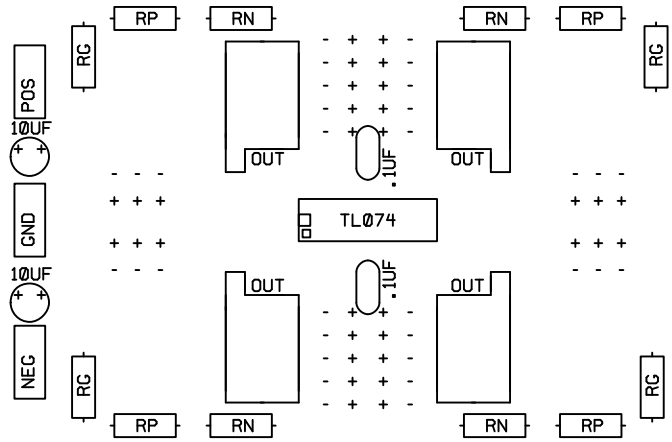
MFOS QUAD SWISS OPAMP KNIFE
